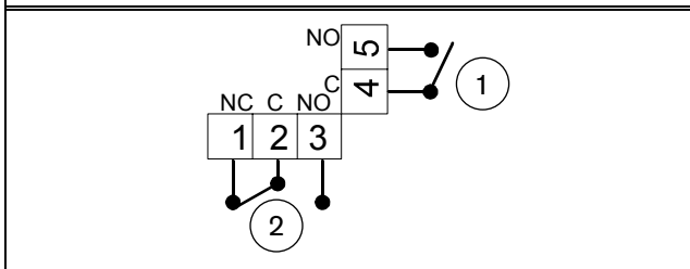
Figure 7: F220-B6C auxiliary/alarm contact wiring
